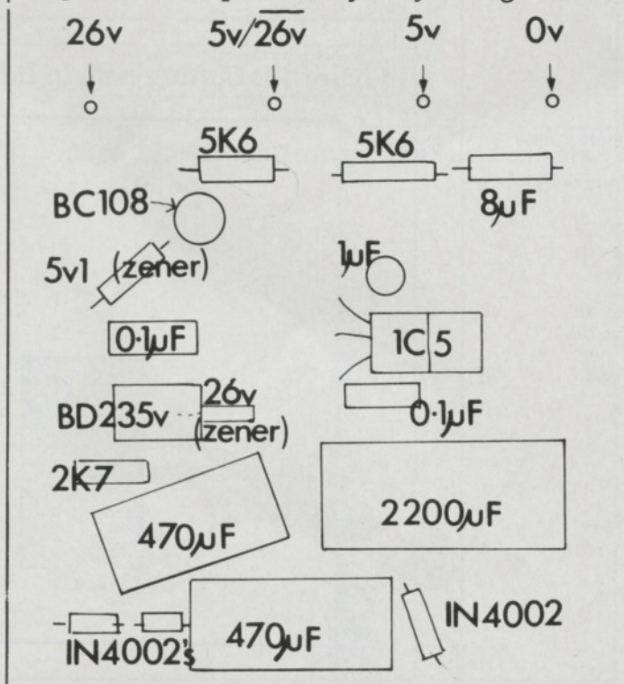
Figure 7: Component layout for large board
